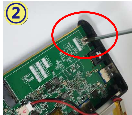
2) Unfasten the M.2 screw
